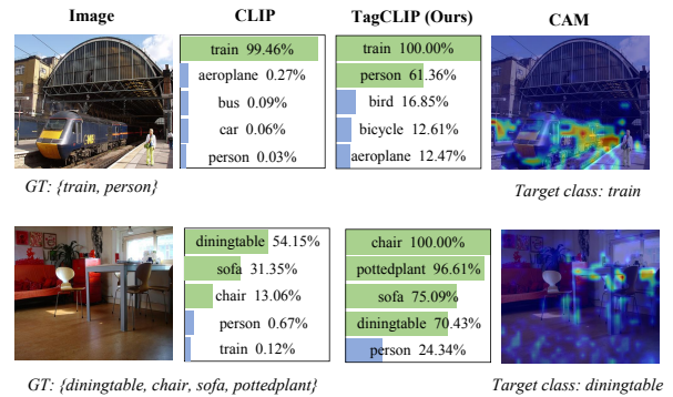
Figure 1: Visualizations of multi-label classification results and CAMs of some target classes. The middle two columns demonstrate that original CLIP (Radford et al. 2021) usually fails to recognize inconspicuous categories while our TagCLIP can identify them well. The last column presents some CAMs of specific classes and indicates that classification mainly depends on some discriminative local features. All results are based on ViT-B/16 and we leverage Grad-CAM (Selvaraju et al. 2017) to obtain CAMs for CLIP.
