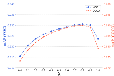
Figure S2: Effect of \lambda on the classification performance on PASCAL VOC 2007 test set and COCO 2014 val set.
