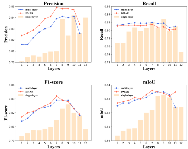
Figure 6: Comparison of single-layer and multi-layer attention refinement in terms of classification and segmentation tasks. For the single-layer setting, each tick i on the x-axis represents merely adopting attention weight in i -th layer. For the multi-layer setting, the i -th x-tick means fusing i -th to 11-th layers attention weights to refine coarse classification scores. We rule out the last attention layer during fusing.
