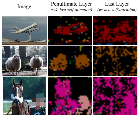
Figure 3: Qualitative results of the patch-level classification upon x_{dense} and x^L outputted by the last two layers of CLIP-ViT respectively. The last self-attention operation breaks spatial information in ViT. We blurred the human face for the ethical consideration.
