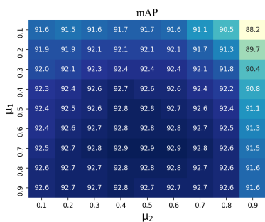
Figure S1: Analysis of \mu_1, \mu_2 on VOC 2007 test set.
