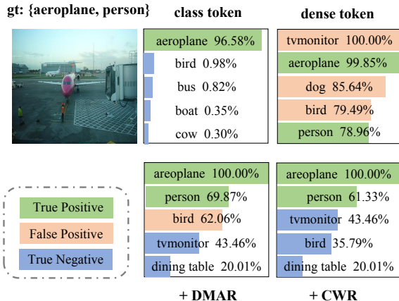
Figure 5: The classification results of class token and dense token and the effect of our proposed modules. We use 0.5 as the threshold by default.
